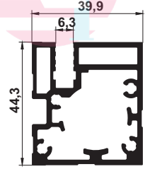
RK-1503 DİKEY BAZA 1,507 kg/m
