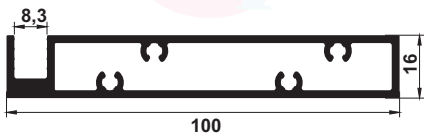
RK-1502 ALT KASA 1,482 kg/m
